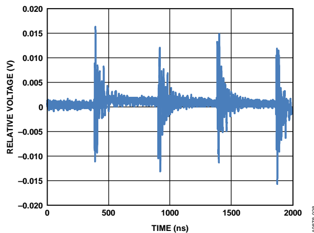
Figure 28. Digital Feedthrough
