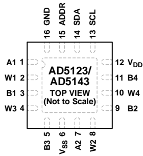
Figure 4. Pin Configuration
