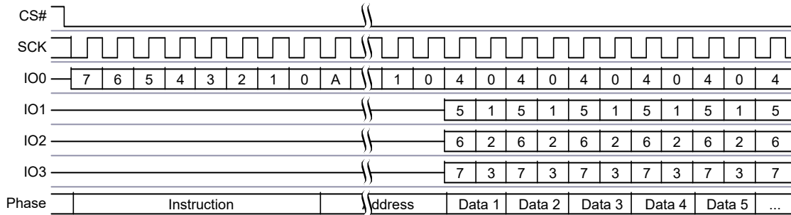
Figure 79. Quad Page Program Command Sequence
