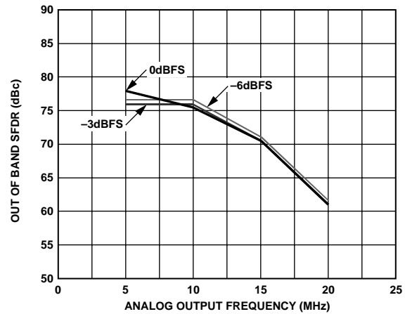
Figure 13. Out-of-Band SFDR, f_{DATA} = 50 MSPS, 8\times Interpolation
