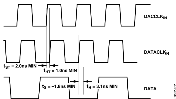
Figure 52. Low Setup and Hold Mode Timing, 1× Interpolation, DCLKPOL = 1
