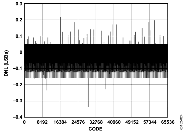
Figure 24. Typical DNL
