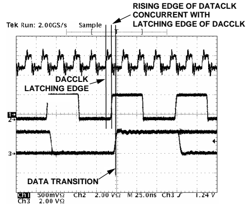
Figure 55. DATAADJ = 1111
