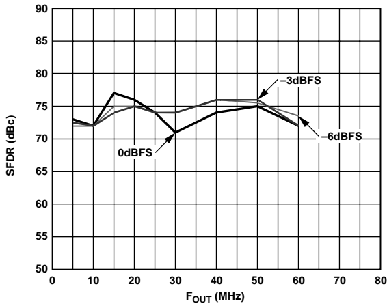
Figure 9. Out-of-Band SFDR, f_{DATA} = 200 MSPS, 2\times Interpolation
