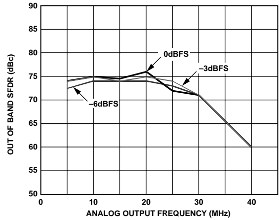
Figure 12. Out-of-Band SFDR, f_{DATA} = 100 MSPS, 4\times Interpolation
