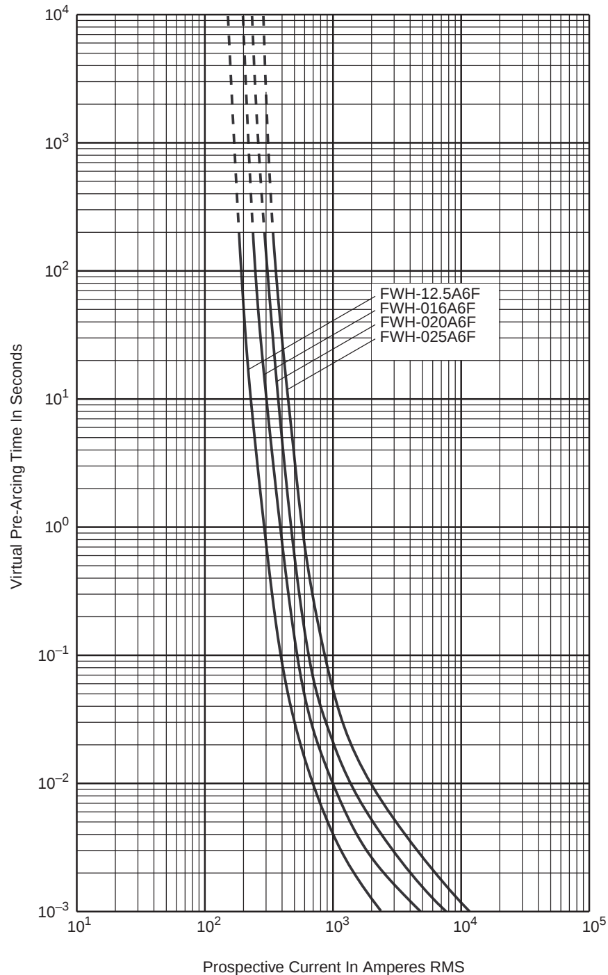
Pre-Arcing Time-Current Characteristic Curves FWH 010A6F-030A6F
