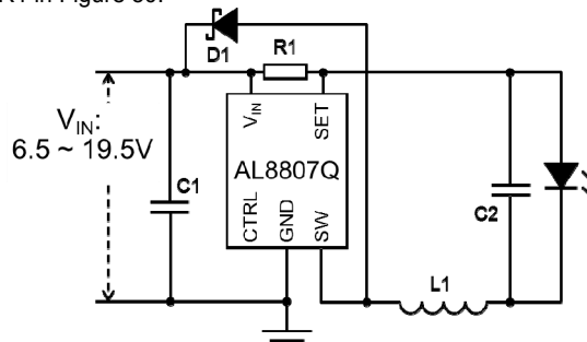
Figure 30 Typical Application Circuit
