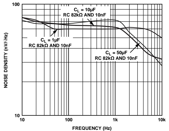
Figure 35. Noise with Compensation Network
