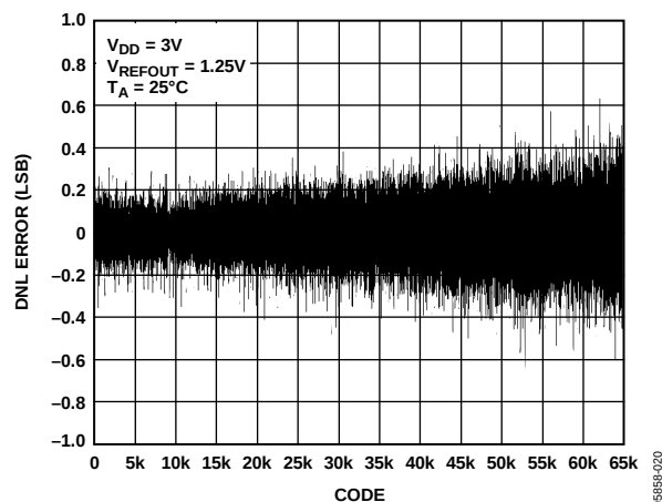
Figure 19. DNL—AD5663R-3
