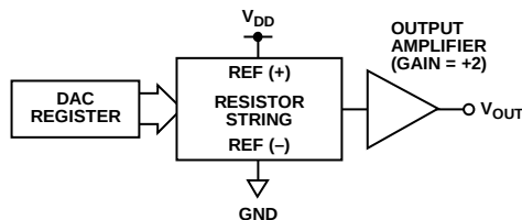
Figure 49. DAC Architecture
