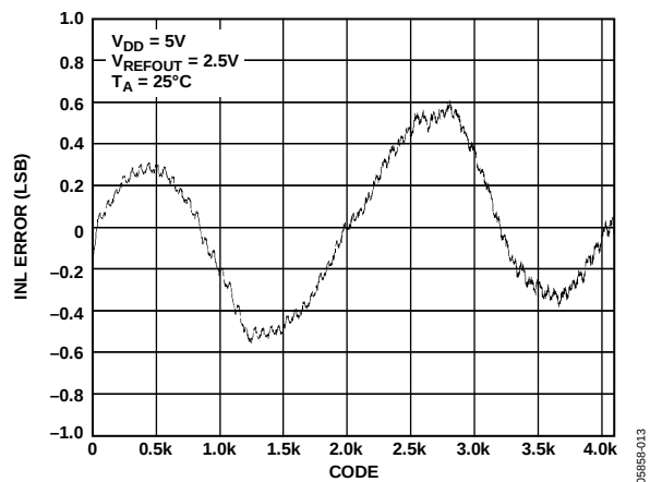
Figure 12. INL—AD5623R-5
