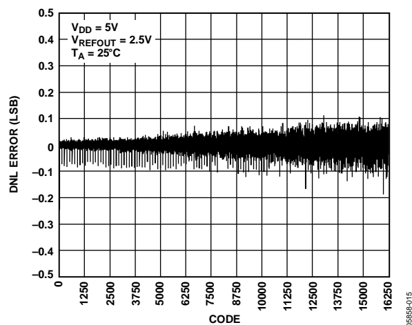
Figure 14. DNL—AD5643R-5
