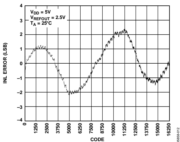
Figure 11. INL—AD5643R-5
