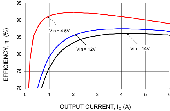
Figure 73. Converter Efficiency versus Output Current.
