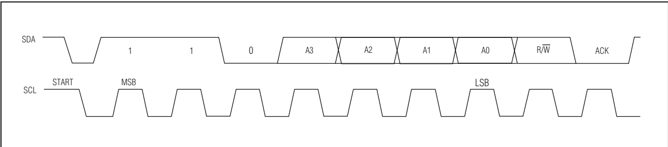
Figure 4. Slave Address
