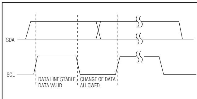
Figure 5. Bit Transfer
