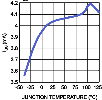
ISS vs. Junction Temperature
