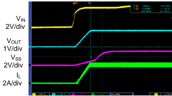
Start Up from V_{IN} ( V_{IN}=5V , V_{OUT}=1.8V , I_{OUT}=4A )
