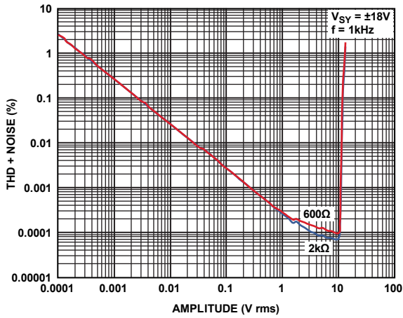
Figure 58. THD + Noise vs. Amplitude
