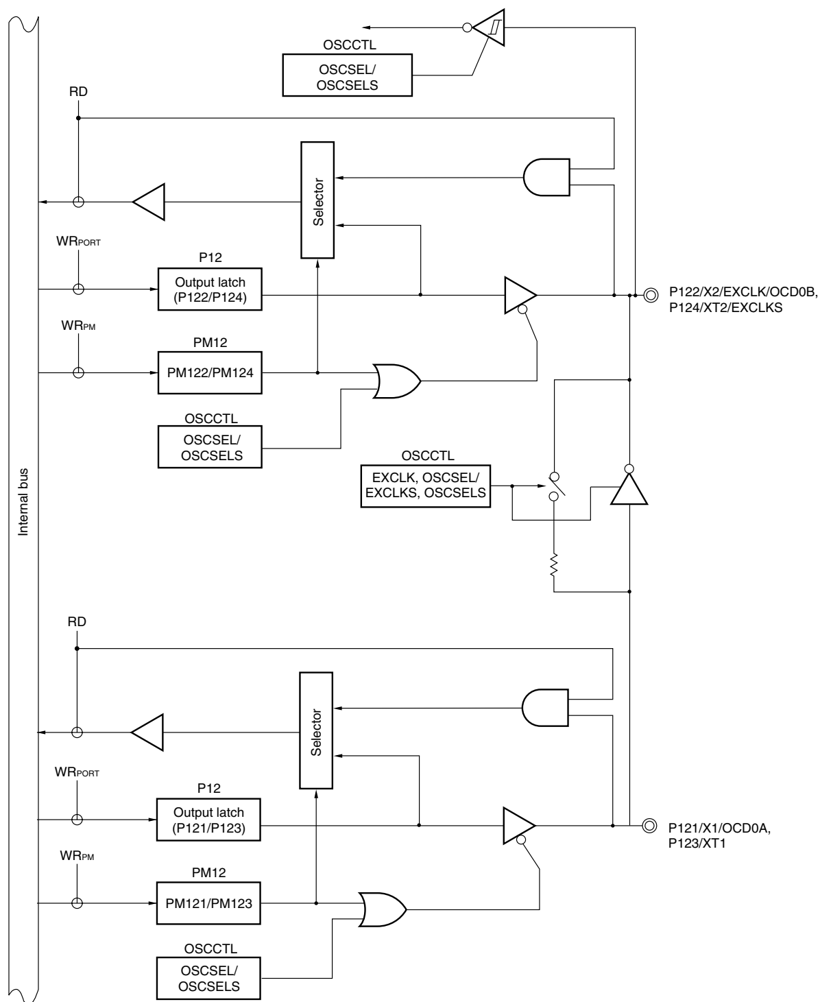
Figure 5-23. Block Diagram of P121 to P124
