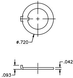
ANTI-ROTATE RING A482 Nickel plated brass 15/32
