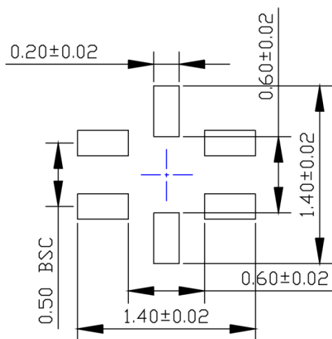
EXPOSED METAL TRACE
