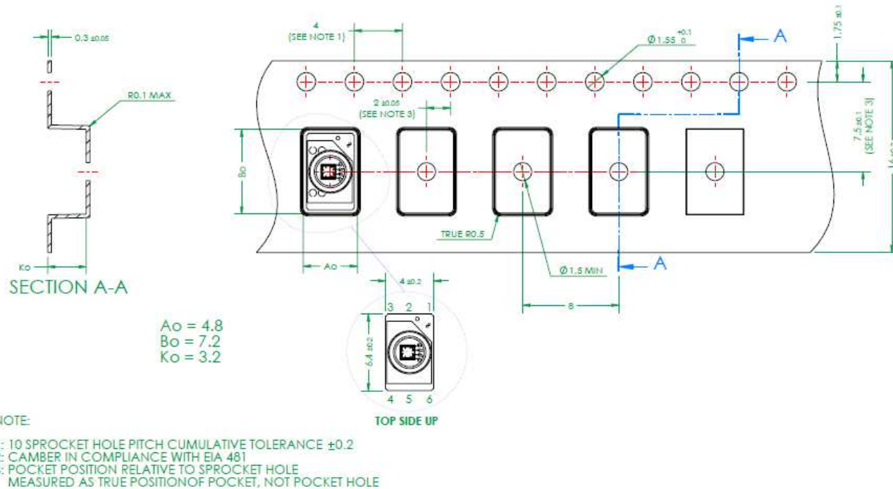
Figure 20: Tape & reel
