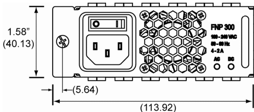
Figure 3 - Mechanical Dimension
