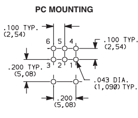
ET21J1ABE2 Horizontal Actuation DPDT
