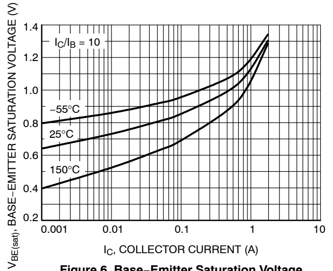
Figure 6. Base-Emmitter Saturation Voltage
