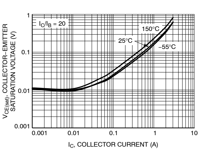
Figure 5. Collector-Emmitter Saturation Voltage
