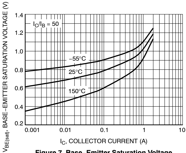
Figure 7. Base-Emmitter Saturation Voltage
