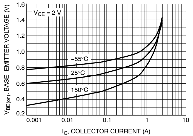
Figure 8. Base-Emmitter Voltage
