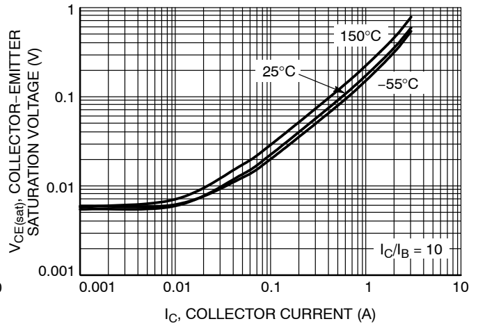
Figure 4. Collector-Emmitter Saturation Voltage
