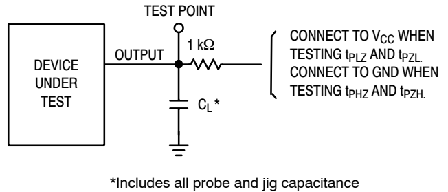
Figure 7. Test Circuit
