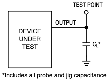
Figure 6. Test Circuit
