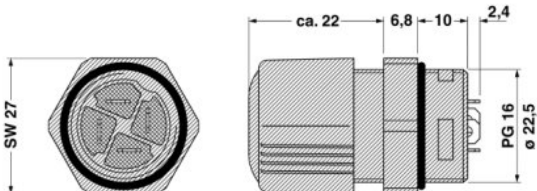
Dimensioned drawing
