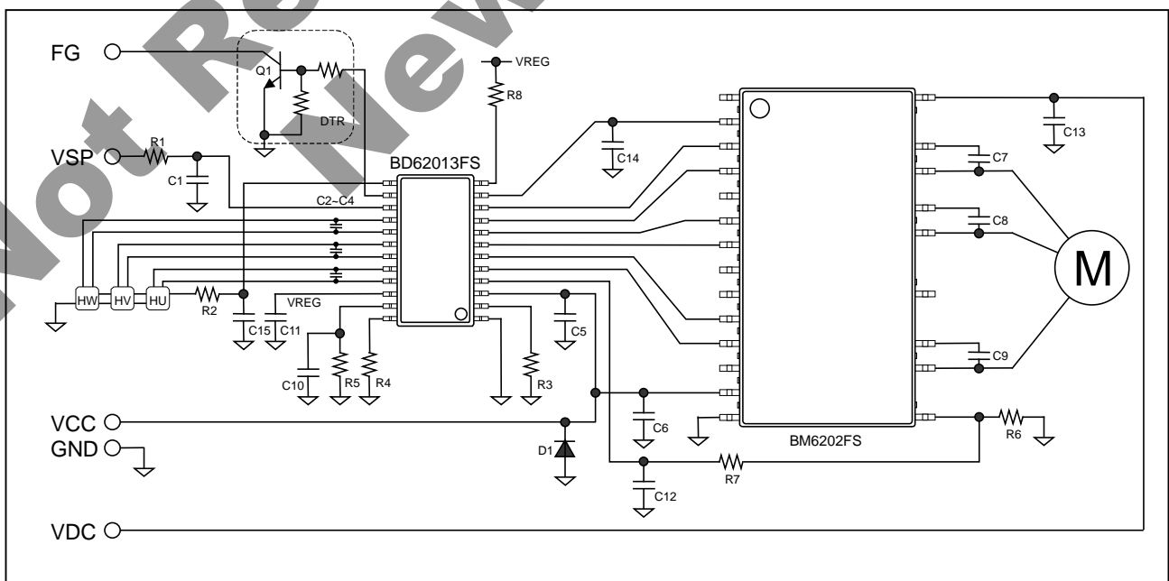
Figure 1. Application circuit example - BD62013FS & BM6202FS
