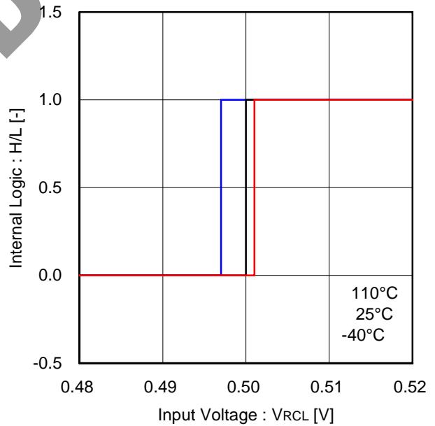
Figure 24. RCL input threshold voltage
