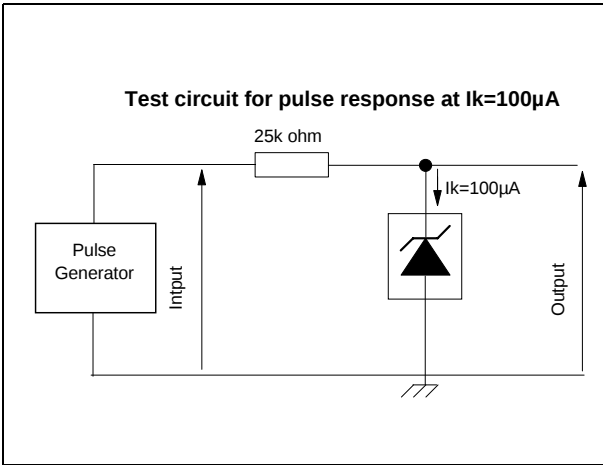
Figure 7. Test circuit for pulse response at I_k=100\mu\text{A}
