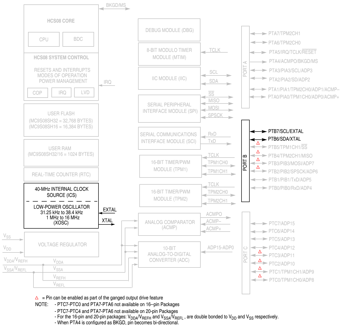
Figure 11-1. MC9S08SH32 Series Block Diagram Highlighting ICS Block and Pins
