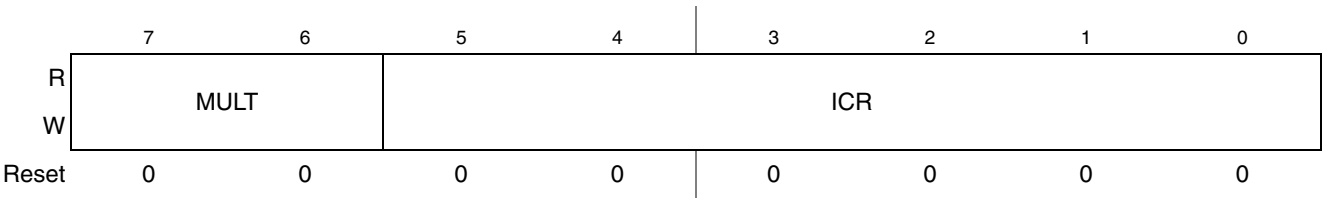
Figure 10-4. IIC Frequency Divider Register (IICF)
