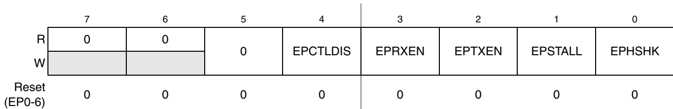
Figure 17-17. Endpoint Control Register (EPCTLn)
