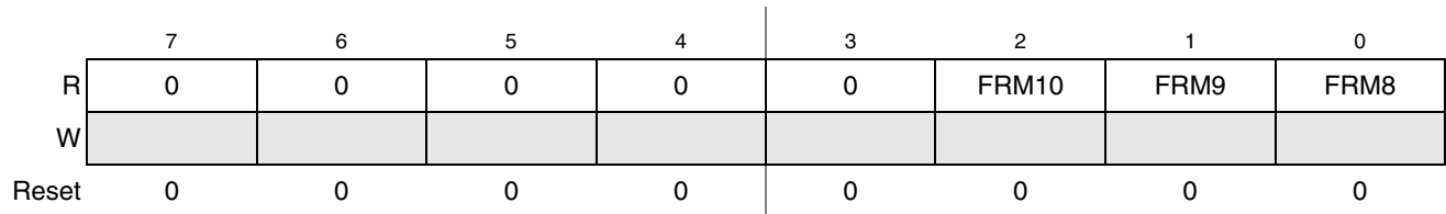
Figure 17-16. Frame Number Register High (FRMNUMH)
