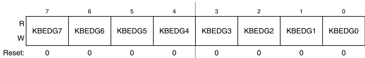
Figure 9-5. KBI Edge Select Register
