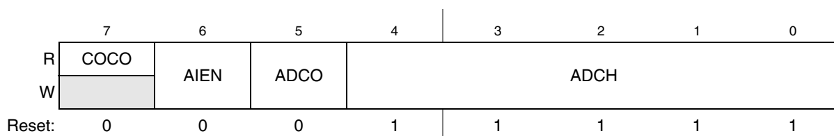
Figure 10-3. Status and Control Register (ADCSC1)
