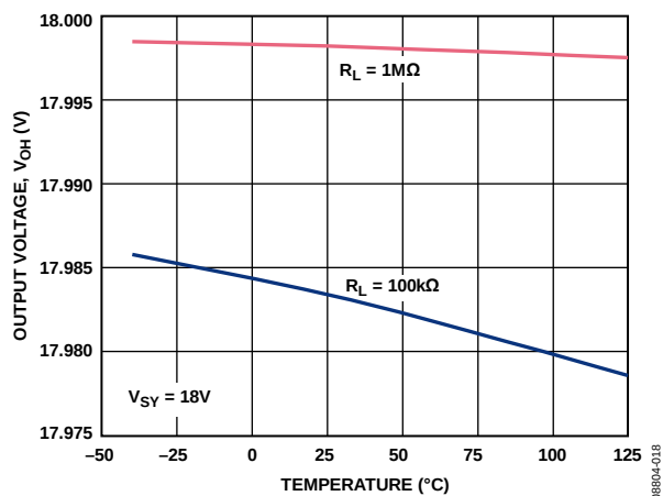
Figure 24. Output Voltage ( V_{OH} ) vs. Temperature
