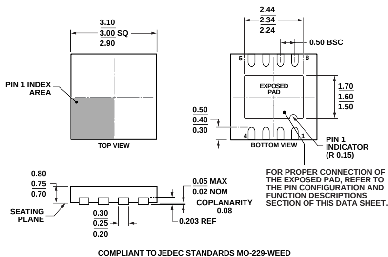
Figure 75. 8-Lead Lead Frame Chip Scale Package [LFCSWP_WD] 3 mm × 3 mm Body, Very Very Thin, Dual Lead (CP-8-11)
