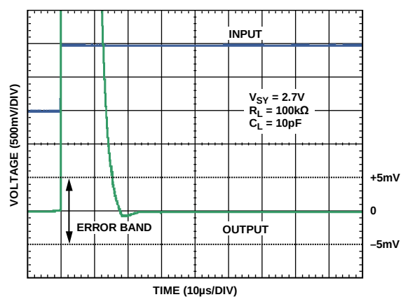
Figure 47. Positive Settling Time to 0.1%
