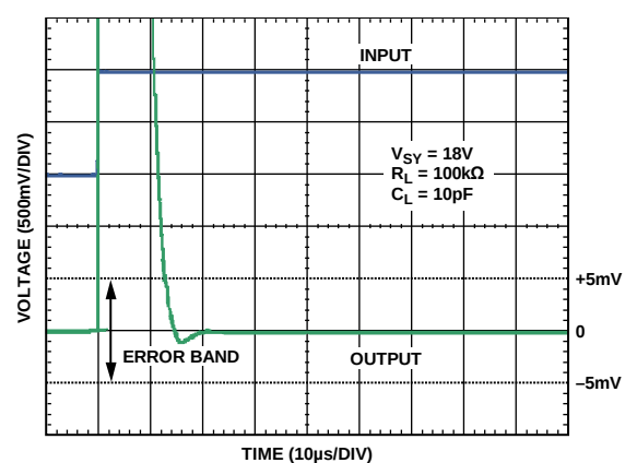
Figure 50. Positive Settling Time to 0.1%
