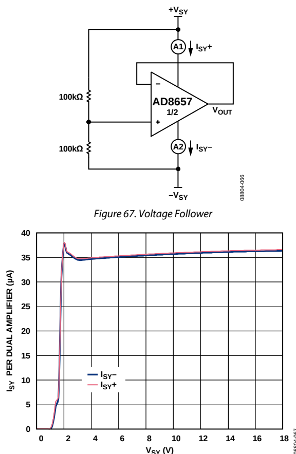
Figure 68. Supply Current vs. Supply Voltage (Voltage Follower)
