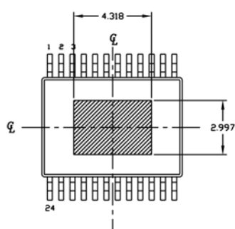
Exposed Pad
