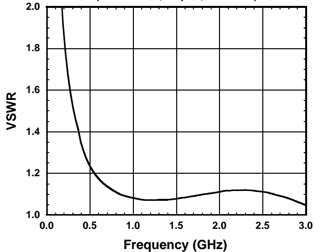
TX-ANT2 VSWR vs. Frequency
