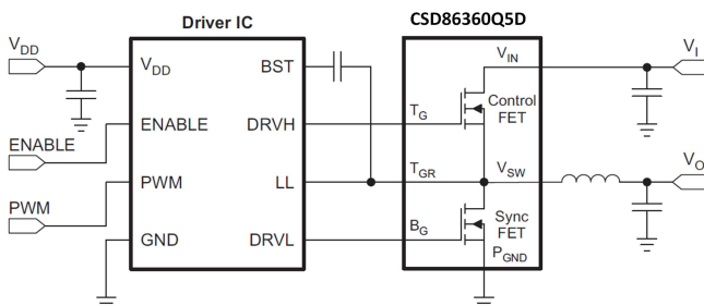
TYPICAL CIRCUIT
