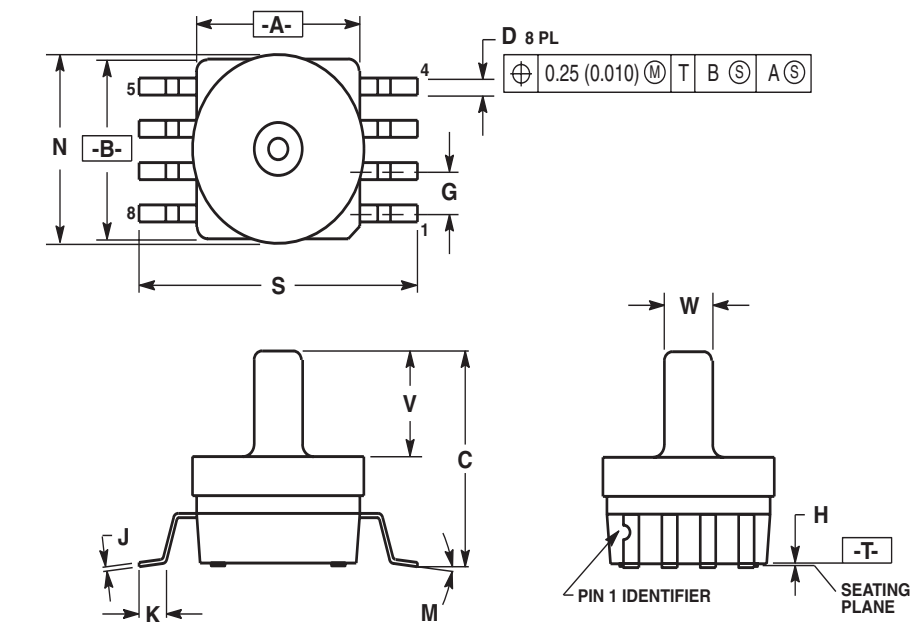
CASE 482A-01 ISSUE A SMALL OUTLINE PACKAGE
