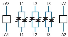
DRHP60x18 (3 controlled legs model) Main Circuit
