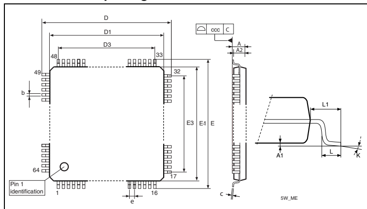
Figure 38. LQFP64 – 10 x 10 mm, 64 pin low-profile quad flat package outline (1)
