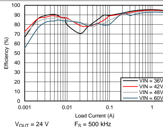
Figure 78. Efficiency
