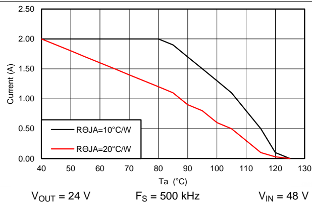
Figure 82. Derating Curve
