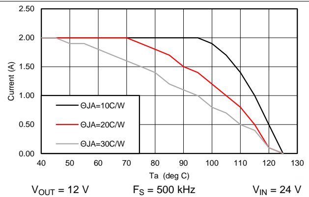
Figure 76. Derating Curve
