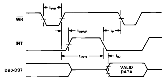
Figure 13. WR-RD Mode Stand-Alone Operation, \overline{CS} = \overline{RD} = 0
