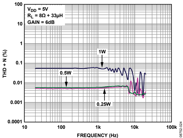
Figure 6. THD + N vs. Frequency, V_{DD} = 5\text{V} , R_L = 8\Omega , Gain = 6 dB
