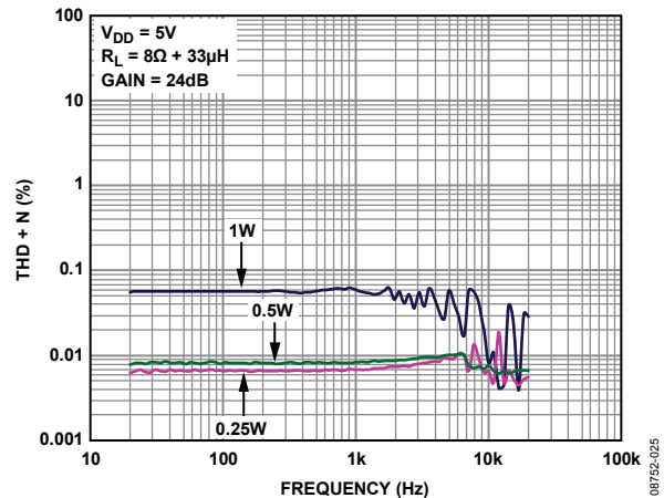
Figure 9. THD + N vs. Frequency, V_{DD} = 5\text{V} , R_L = 8\Omega , Gain = 24 dB
