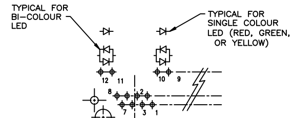
LED SCHEMATIC
