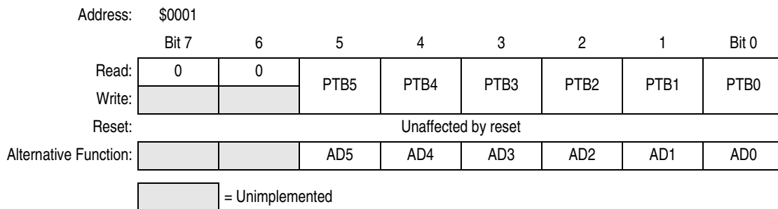
Figure 16-6. Port B Data Register (PTB)
