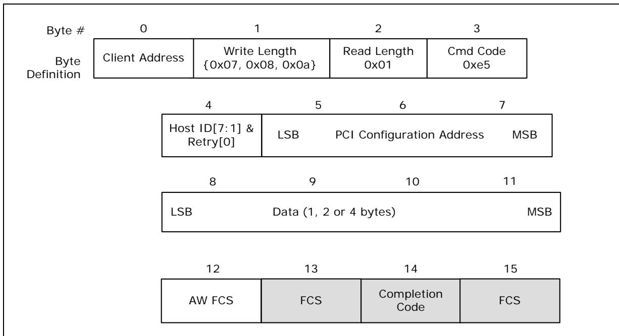
Figure 2-48. WrPCIConfigLocal()
