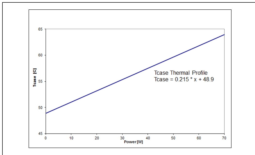
Figure 5-15. Tcase: 8-Core 70W Thermal Profile 1U
