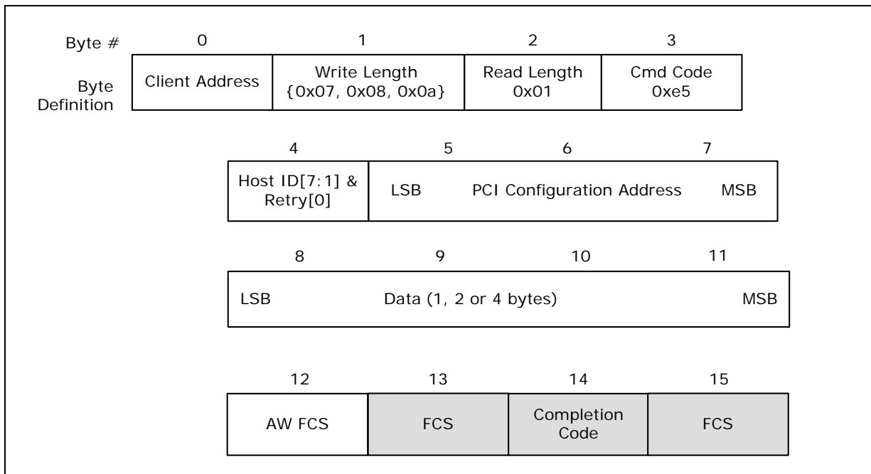
Figure 2-48. WrPCIConfigLocal()
