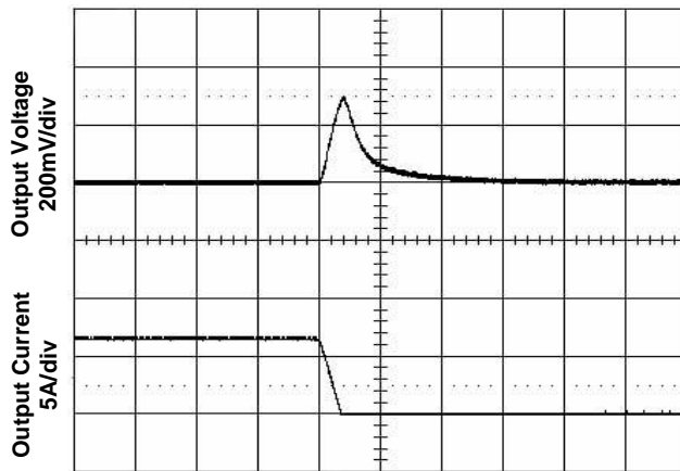
Figure 7. Transient Load Response Top: Output voltage deviation Bottom: Load current step (-25% full load) Test Cond.: Output current at 20A 50% full load, typical Vin, slew rate 0.1A/µs
