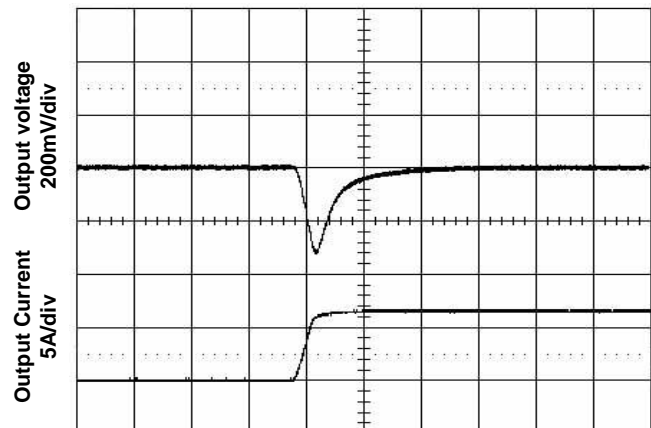
Figure 8. Transient Load Response Top: Output voltage deviation Bottom: Load current step (+25% full load) Test Cond.: Output current at 20A 50% full load, typical Vin, slew rate 0.1A/µs
