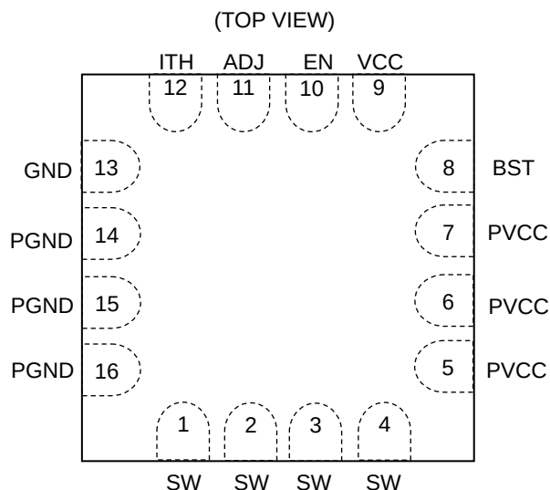
Figure 2. Pin Configuration
