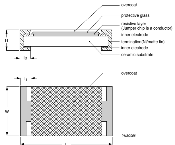
Fig. 2 Chip resistor outlines
