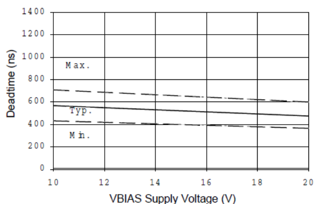
Figure 11B. Deadtime vs Voltage
