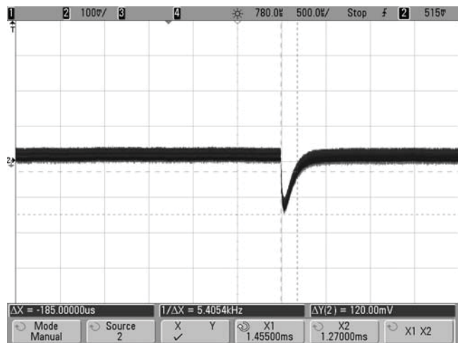
Step Load Transient Response (Vin=48V, Vout=nominal, Load=0, Iout=50% to 75% of full load, Ta=+25°C.) Trace 1=Vout, 100 mV/div., 500 µS/div.
