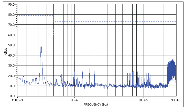
Graph 5. Conducted emissions performance, Positive Line, CISPR 22, Class A, full load
