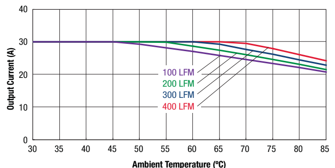
UEE-3.3/30-D48 Maximum Current Temperature Derating at Sea Level (Vin = 48V, with baseplate. Airflow direction is transverse from +Vin to -Vin.)
