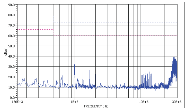
Graph 6. Conducted emissions performance, Negative Line, CISPR 22, Class A, full load
