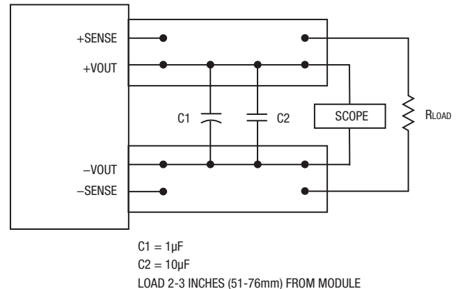
Figure 7. Measuring Output Ripple and Noise (PARD)
