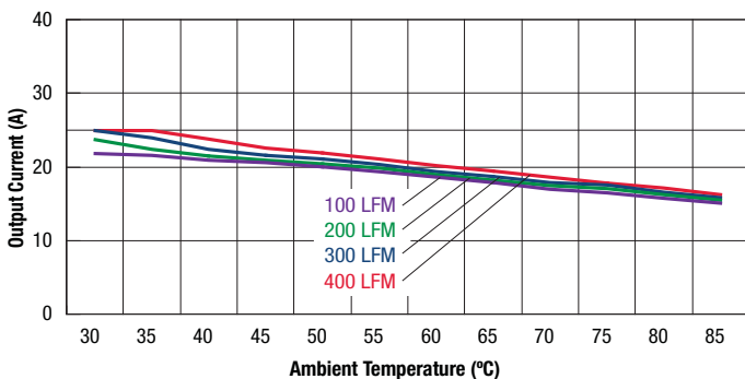
UEE-3.3/25-D48 Maximum Current Temperature Derating at Sea Level (Vin = 48V, no baseplate. Airflow direction is transverse.)
