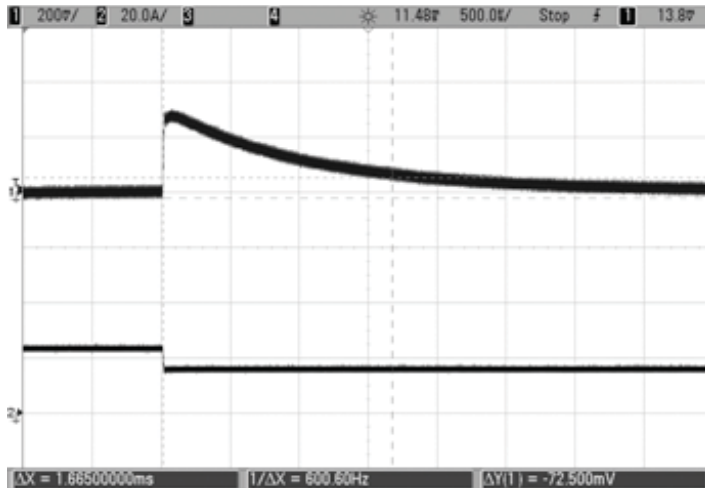
Step Load Transient Response ( V_{in} = 48V , V_{out} = \text{nom} , C_{load} = 1\mu F \parallel 10\mu F , I_{out} = 75\% \text{ to } 50\% of full load, T_a = +25^\circ C ) Ch1 = Vout, Ch2 = Iout
