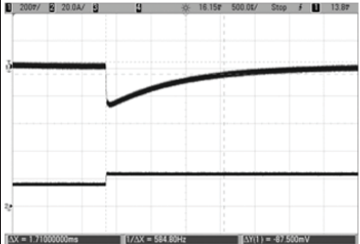
Step Load Transient Response ( V_{in} = 48V , V_{out} = \text{nom} , C_{load} = 1\mu F \parallel 10\mu F , I_{out} = 50\% \text{ to } 75\% of full load, T_a = +25^\circ C ) Ch1 = Vout, Ch2 = Iout
