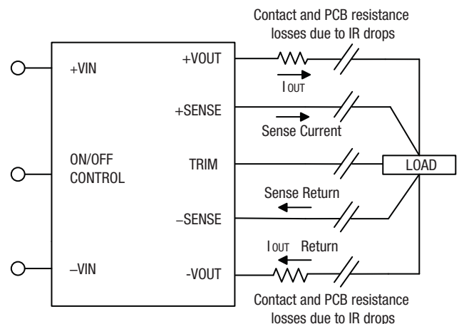
Figure 8. Remote Sense Circuit Configuration
