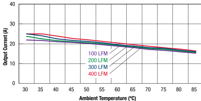
UEE-3.3/25-D48 Maximum Current Temperature Derating at Sea Level (Vin = 48V, no baseplate. Airflow direction is longitudinal, from Vin to Vout.)
