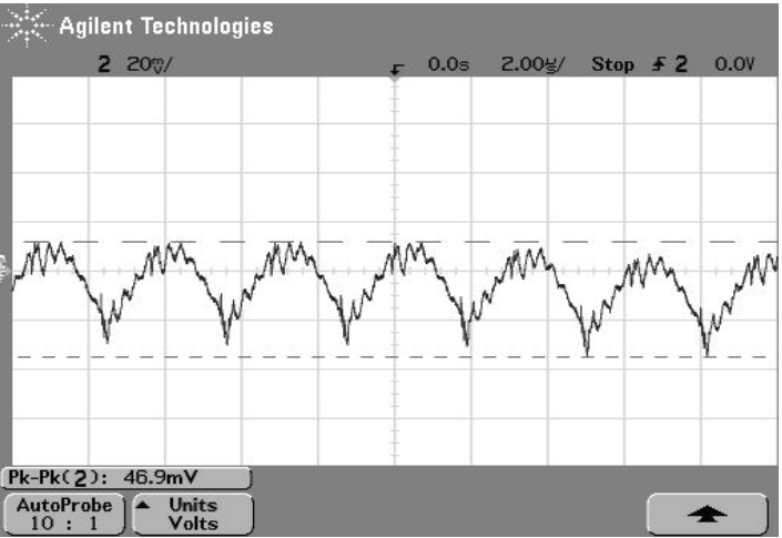
Output Ripple and noise (Vin=48V, Vout=nom., Iout=0A, Cload=0, Ta=+25° C., ScopeBW=20Mhz)
