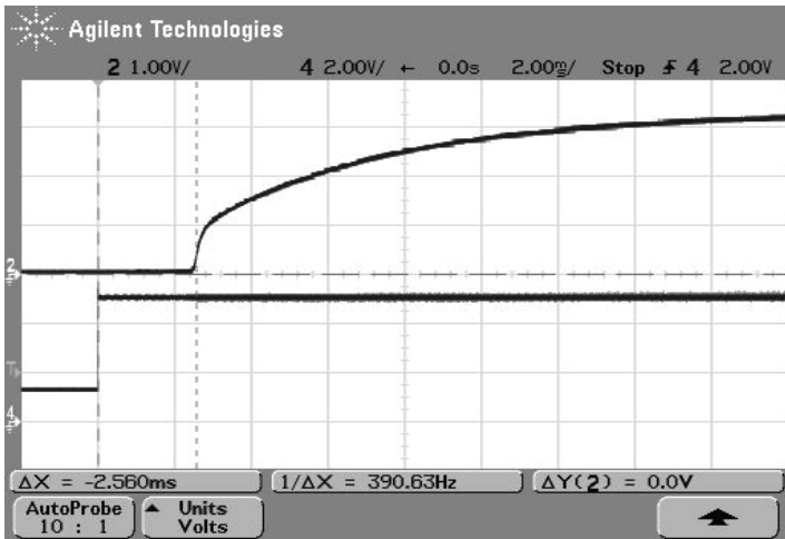
Power On Start Up (Vin=48V, Vout=nom., Iout=15A, Cload=7500uF, Ta=+25° C., ScopeBW=20Mhz, Trace 2=Vout, Trace 4=Enable)
