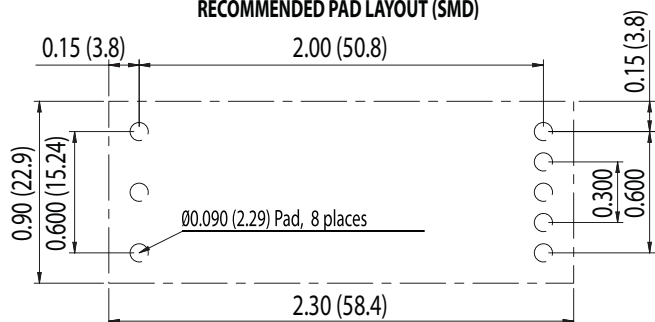
RECOMMENDED PAD LAYOUT (SMD)
