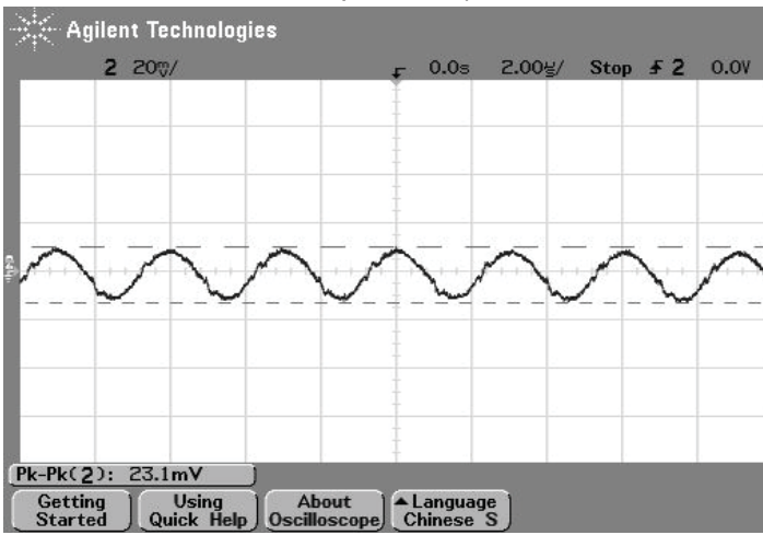
Output Ripple and noise (Vin=48V, Vout=nom., Iout=30A, Cload=0, Ta=+25° C., ScopeBW=20Mhz)
