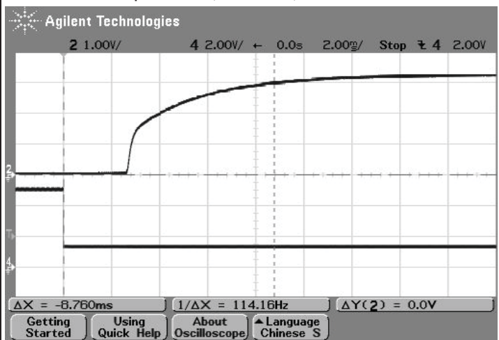
On/Off Enable Delay (Vin=48V, Vout=nom., Iout=30A, Clod=10uF, Ta=+25° C., ScopeBW=20Mhz, Trace 2=Vout, Trace 4=Enable.)
