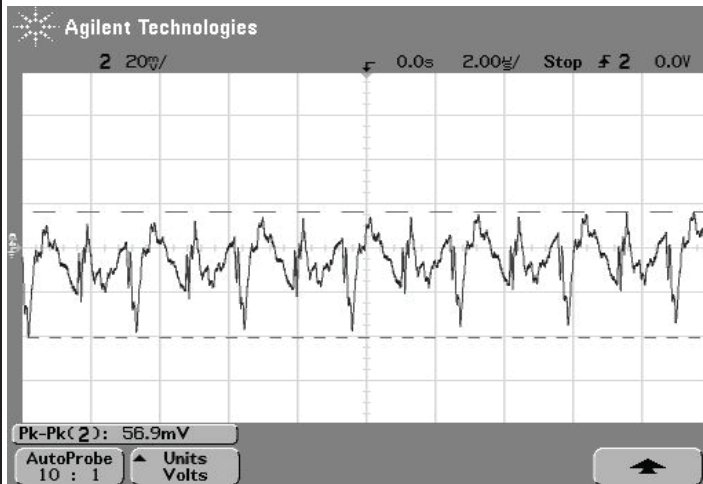
Output Ripple and noise (Vin=48V, Vout=nom., Iout=15A, Cload=0, Ta=+25° C., ScopeBW=20Mhz)
